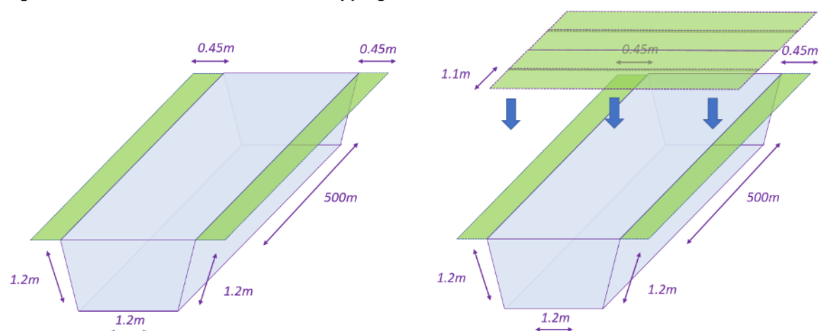
Figure 4: CC8 anchor trenches and overlapping sections
