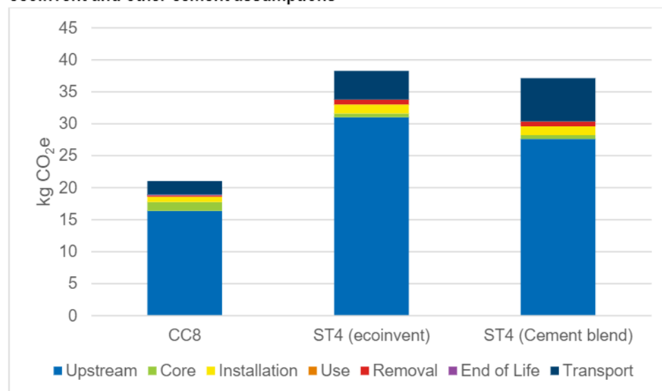
Figure 10: Global warming potential per m 2 of channel, by life cycle stage, comparing ST4 under ecoinvent and other cement assumptions
